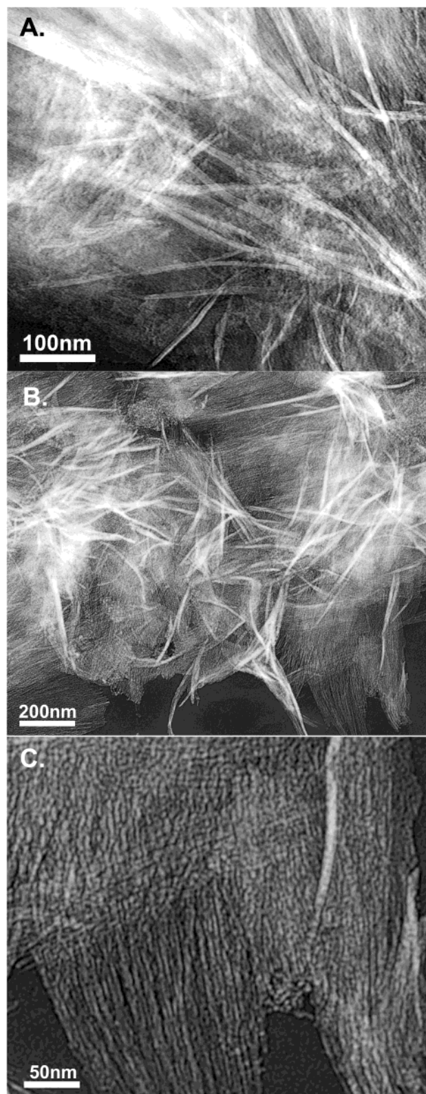
Figure 4. TEM images of (A) surfactant–boehmite mesophase (MSU-S/B) made at 70 °C from \text{Al}_{13} oligocations and Pluronic P84 surfactant, and (B and C) the corresponding MSU- \gamma phase with crystalline \gamma - \text{Al}_2\text{O}_3 walls formed through calcination of the MSU-S/B mesophase at 550 °C for 4 h.
