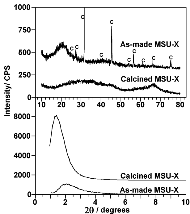
Figure 1. XRD patterns in the 2 \text{ \AA} ranges 1\text{--}10^\circ (lower patterns) and 10\text{--}80^\circ (upper patterns) for as-made ( 70 °C) and calcined ( 550 °C) MSU-X mesostructures assembled from \text{Al}_{13} oligocations and the triblock surfactant (\text{EO})_{19}(\text{PO})_{43}(\text{EO})_1 (Pluronic P84). The sharp reflections labeled “C” in the pattern of the as-made mesostructure arise from the \text{NH}_4\text{Cl} byproduct.
