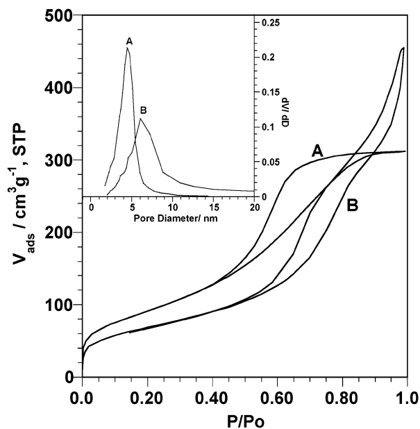
Figure 6. N 2 adsorption–desorption isotherms and BJH pore size distributions (inset) for MSU- \gamma aluminas derived from Pluronic P84 surfactant and (A) Al(NO 3 ) 3 and (B) Al 13 oligocations as the aluminum reagent. The assembly temperature in each case was 70 °C.
